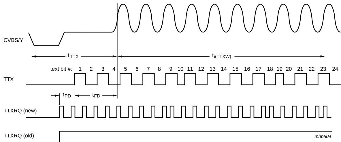
Fig 23. Teletext timing
