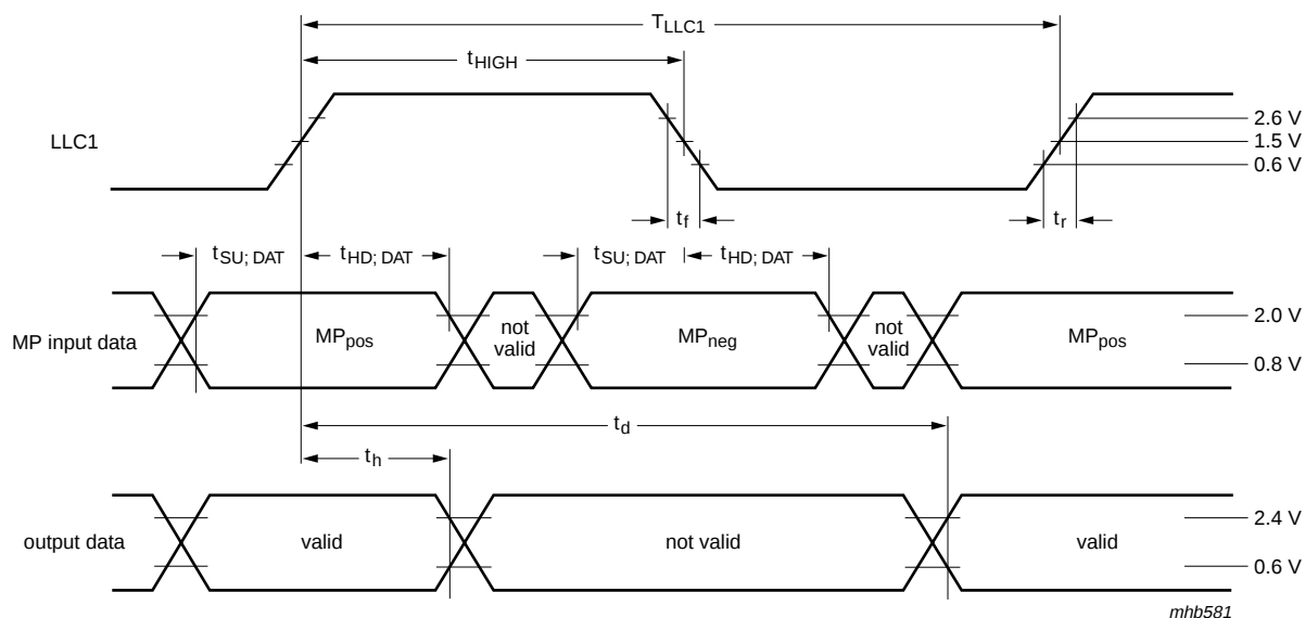
Fig 20. Clock data timing
