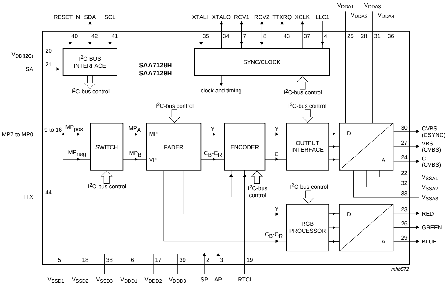
Fig 1. Block diagram
