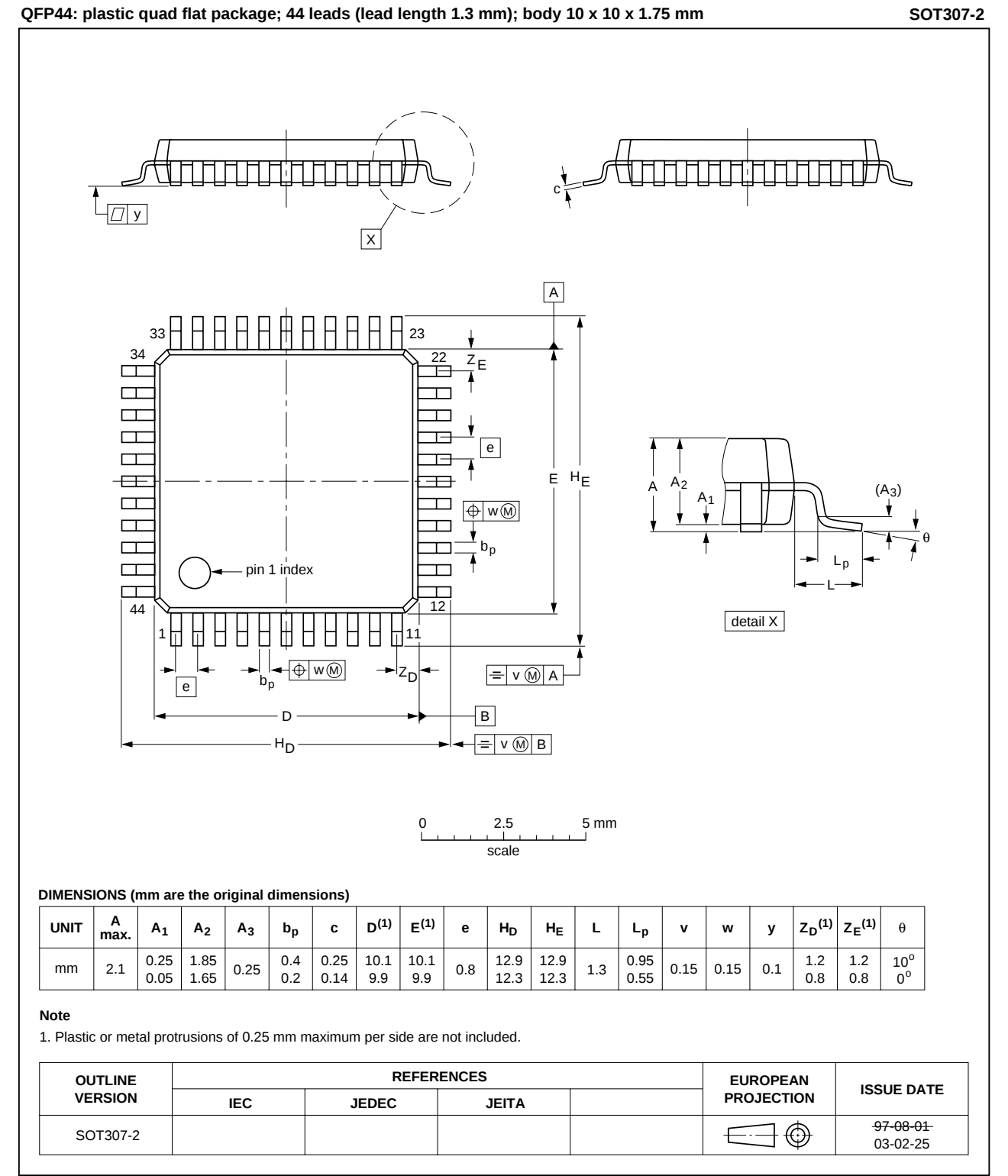
Fig 25. Package outline SOT307-2 (QFP44)
